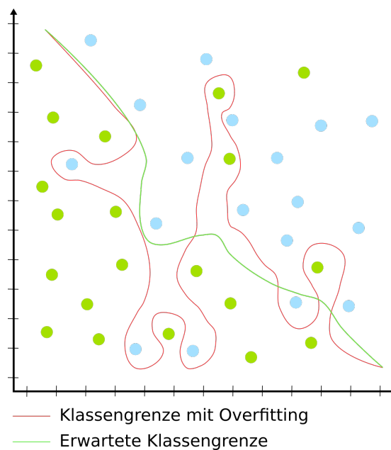
Abbildung 3: Overfitting
